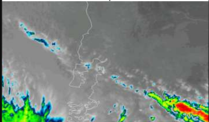
Calbuco Volcanic Eruption from GOES-13
